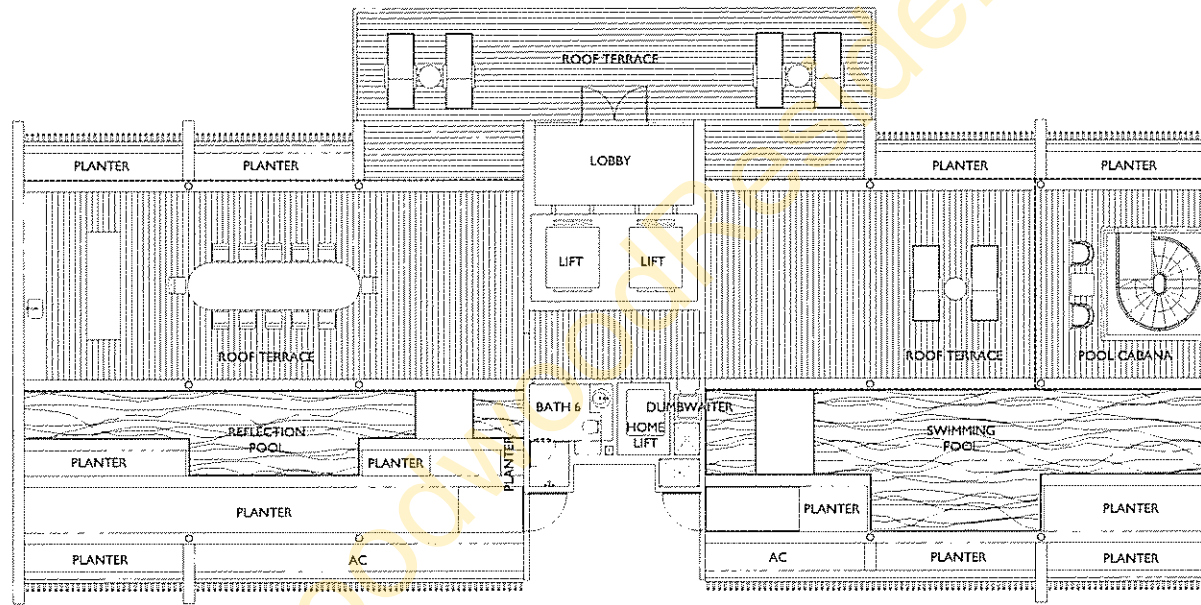
Upper Level
